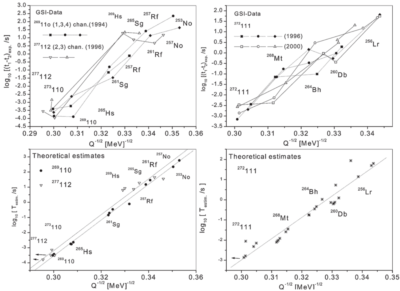
Fig. 1 – Summary of the \alpha -decay data obtained by Hofmann et al. [37–39] and estimated \alpha -half-lives and emission energies for the nuclei Z = 110 – 112 and their \alpha descendants.
