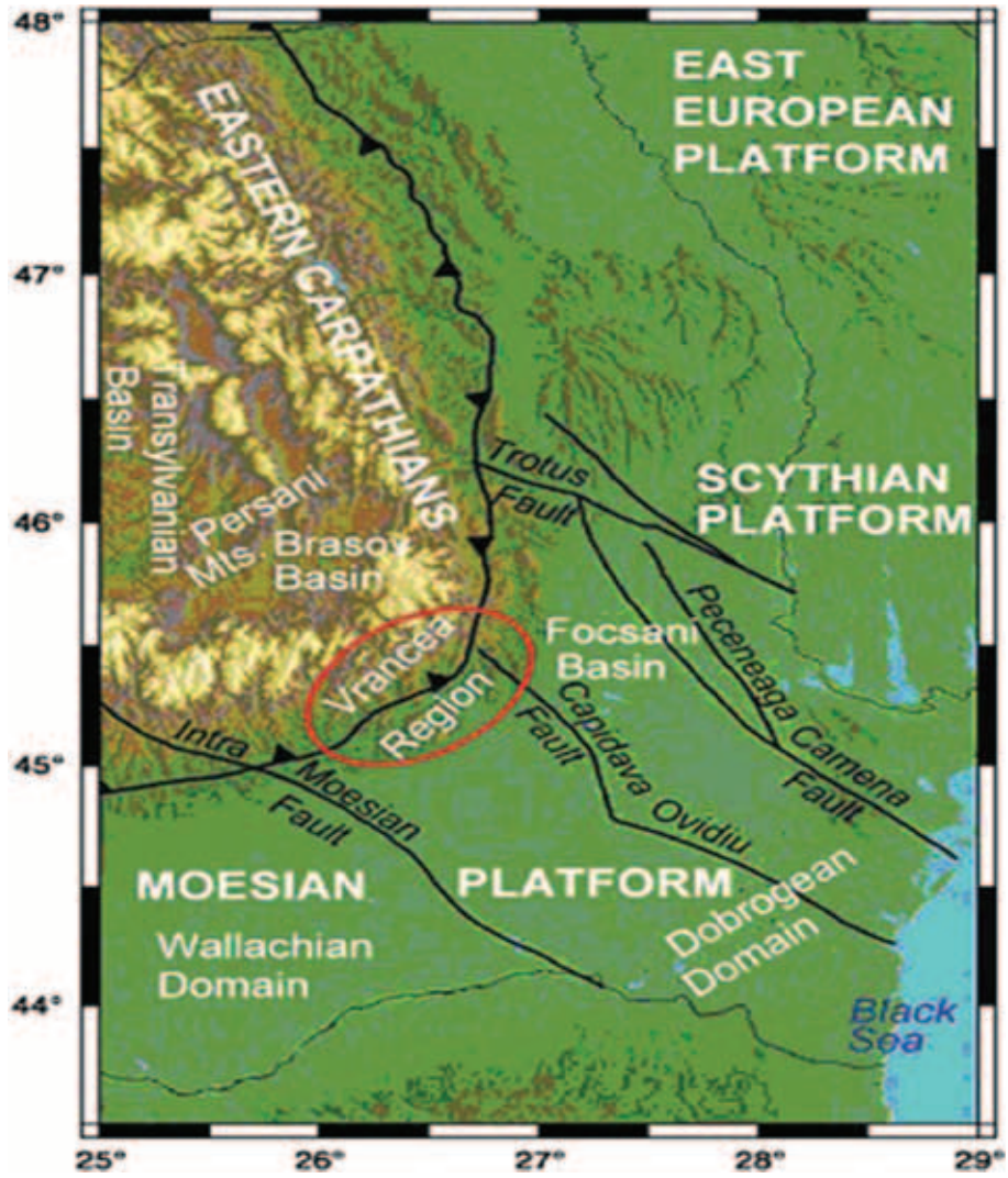
Fig. 1 – Main tectonic units and major faults in the Vrancea zone [5].
