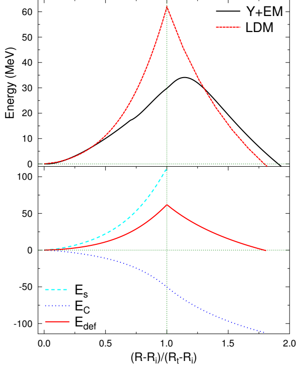
Fig. 1 – TOP: potential barrier for emission of ^{34}\bar{S}i from ^{242}\bar{C}m calculated within LDM (red) Y+EM (black). BOTTOM: two main terms of the LDM barrier: surface energy (dashed line cyan) and Coulomb energy (dotted line blue).
