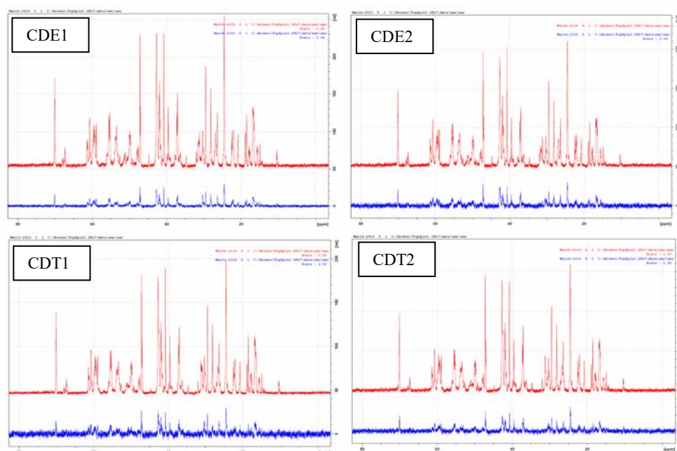
Fig. 3 – The ^{13}\text{C} -NMR spectra of collagen fragments from old bone samples.
