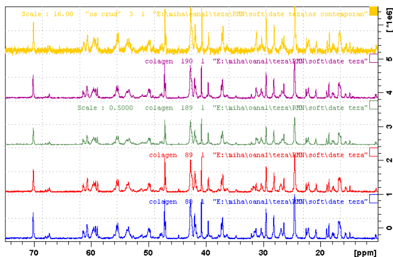
Fig. 2 – ^{13}\text{C} -NMR spectra obtained for collagen: from contemporary collagen (yellow) and collagen extracted from old bones samples.
