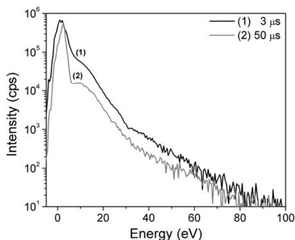
Fig. 6 - Time averaged ion energy distribution of \text{Cu}^{1+} for selected pulse durations.
