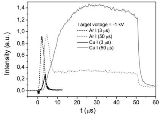
Fig. 4 - Time evolution of Ar I and Cu I atomic spectral line intensities during on pulse of 3 and 50 \mu\text{s} , respectively.
