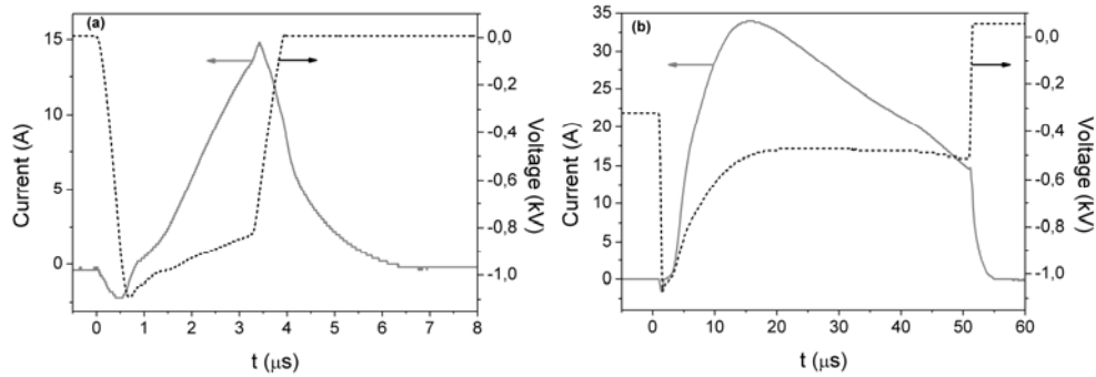
Fig. 2 - Discharge current intensity and voltage waveforms for: (a) short pulses of 3 \mu\text{s} and (b) long pulses of 50 \mu\text{s} .
