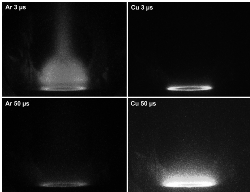
Fig. 3 - On-pulse fast ICCD images registered at 3 \mu\text{s} and 50 \mu\text{s} respectively, with red (Ar) and green (Cu) bandpass optical filters.
