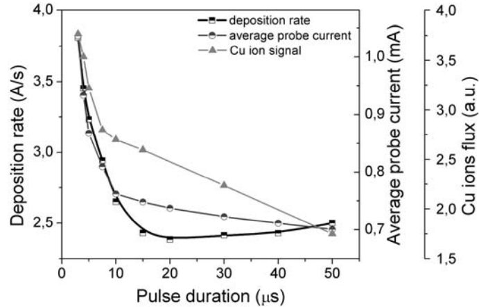
Fig. 5 - Deposition rate, average probe current and Cu ions flux dependence on the pulse duration.
