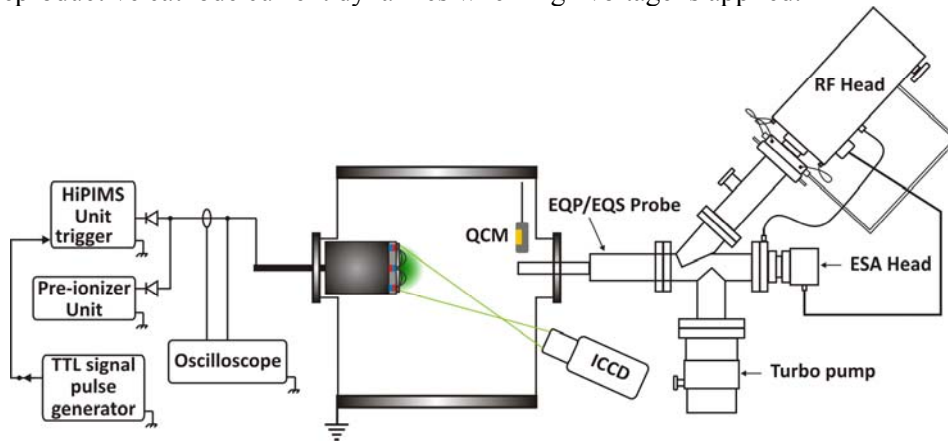
Fig. 1 - Schematic view of the experimental setup including the HiPIMS system, quartz crystal microbalance (QCM), ICCD camera (ICCD), and mass spectrometer.
