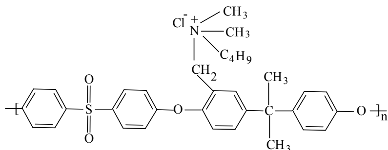
Scheme 1 - Chemical structure of quaternized polysulfone involved in the study.
