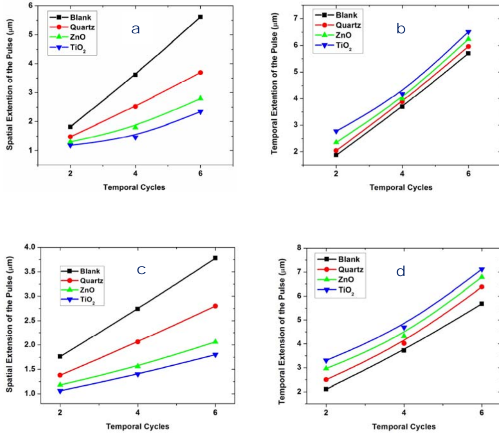
Fig. 3. Spatio-temporal analysis of the TFP extension for all four media investigated. a) Spatial extension of TFP at f\# = 3.75 ; b) Temporal extension of TFP at f\# = 3.75 ; c) Spatial extension of TFP at f\# = 0.83 ; d) Temporal extension of TFP at f\# = 0.83 .
