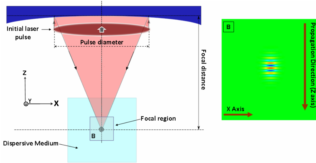
Fig. 1. Schematic design of the pulse focusing and the electromagnetic field distribution in focus in the case of an extended source illustrating the Gaussian beam E_y distribution in the (xz) plane.
