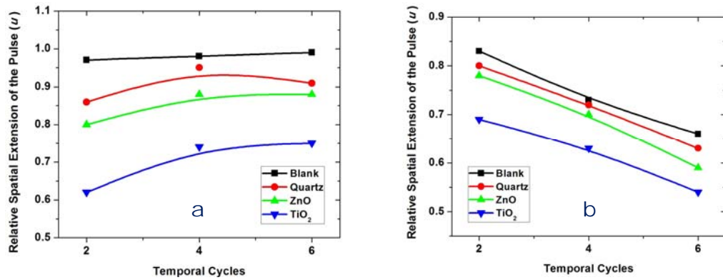
Fig. 4. Relative spatial extension of the pulse for all four media investigated in the case of pulse duration variation at a) f\# = 3.75 and b) f\# = 0.83 .
