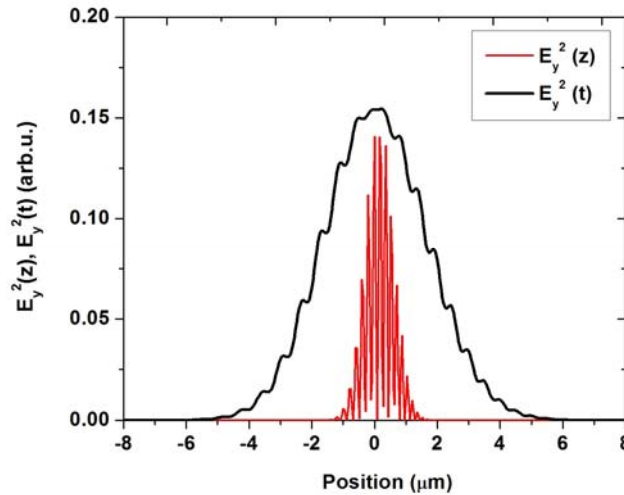
Fig. 2. Relation between spatial and temporal envelopes for the square of the electric field in the case of no dispersive medium at 2 cycles pulse duration and an f -number of 3.75. The full width at half maximum of the spatial envelope is 1.85 \mu\text{m} while the temporal envelope has 2.8 \mu\text{m}/c duration, where c is the speed of light.
