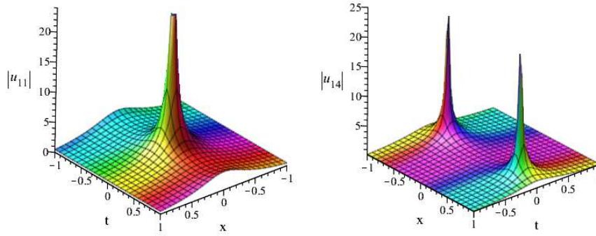
Fig. 1 – Snapshots of traveling wave solutions u_{11} and u_{14} of (13) for c = 5 and k = 2 .
