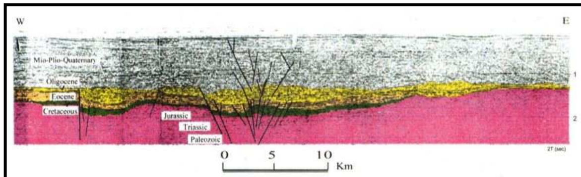
Fig. 7 - P 11-Seismic line over Nistru Fault after [15]. See Fig.5
