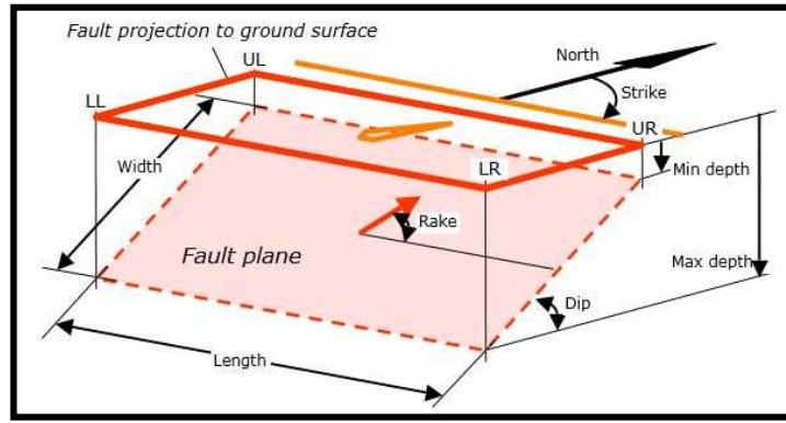
Fig.3 - Schematic representation of an Individual Seismogenic Source and its characteristics [1]
