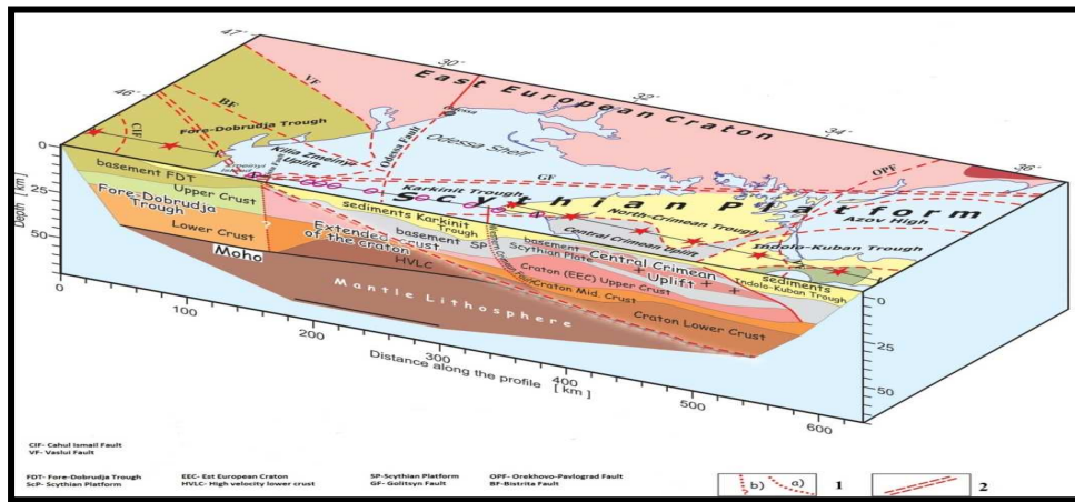
Fig. 8 - Dobro 5 profile. Interpreted velocity model vs surface geology. 1. Deep Faults. a) clearly distinguished in the seismic section and related to surface fault-Western Crimea Fault; b) not clearly distinguished on seismic section but related with surface fault - Nistru Fault. 2. Crustal fault between the Scythian Platform and Est European Craton associated with the Golitsyn Fault (GF) on the surface. After [33]
