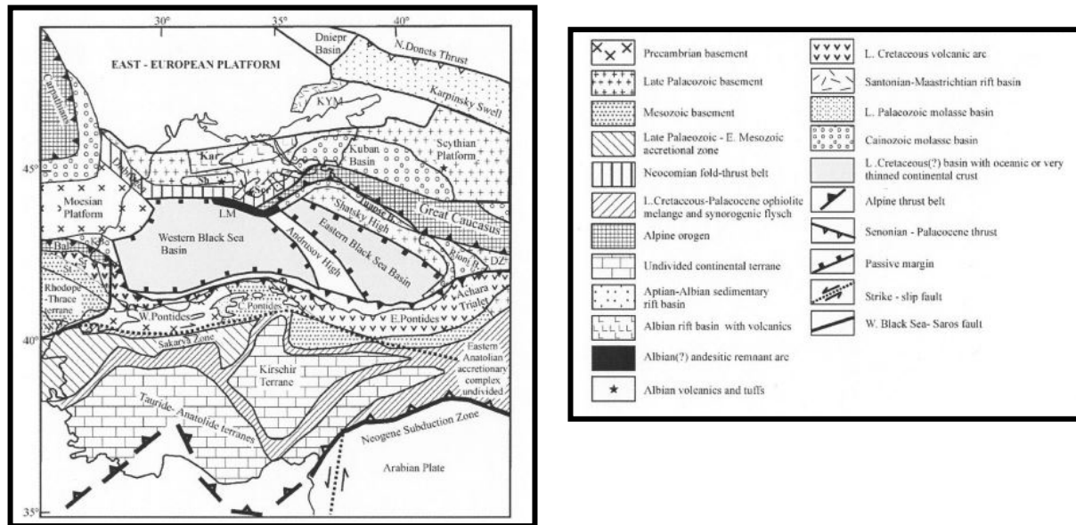
Fig.1 - Geotectonic map of the Black Sea basin. A: Alma Basin, Bal: Balkanides, Dz:Dzirula, G: Guriy basin, K: Kamchia foreland Basin, Kar: Karkinit trough, KYM: Konka-Yaly-Molochanaya graben, Scr: South Crimea Orogen, Sh: Shtormovaya graben, Sr:Srednogie, St:Strandzha, WBS: West Black Sea-Saros fault [23]
