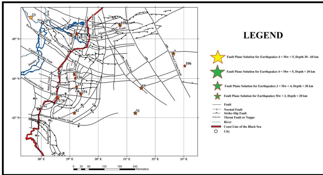
Fig.4 - Earthquakes with fault plane solutions on the tectonic background. Numbers indicate the current event number in Table 3. Tectonics after [15] and [29]
