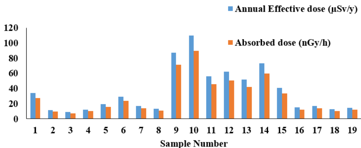
Figure 4. Annual effective dose and absorbed dose values according to sample number.
