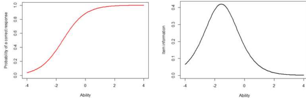
Fig. 10 – Characteristic curve (left) and information curve (right) of Item 8
