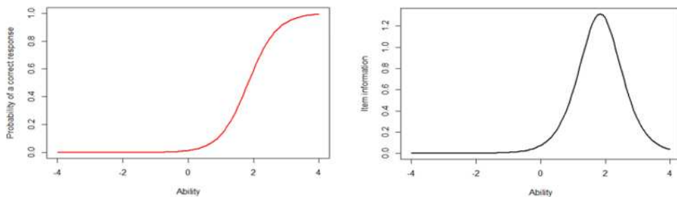
Fig. 13 – Characteristic curve (left) and information curve (right) of Item 14
