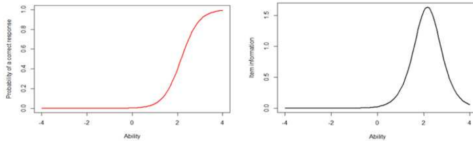
Fig. 12 – Characteristic curve (left) and information curve (right) of Item 4
