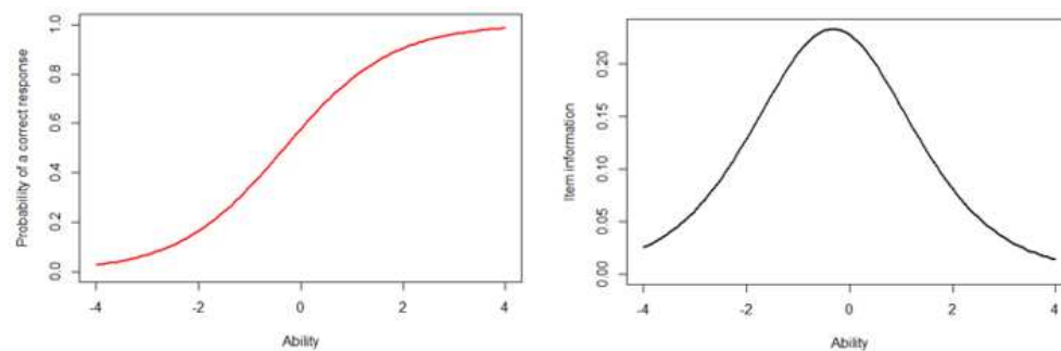
Fig. 11 – Characteristic curve (left) and information curve (right) of Item 12
