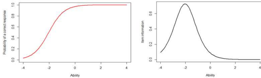
Fig. 8 – Characteristic curve (left) and information curve (right) of Item 3
