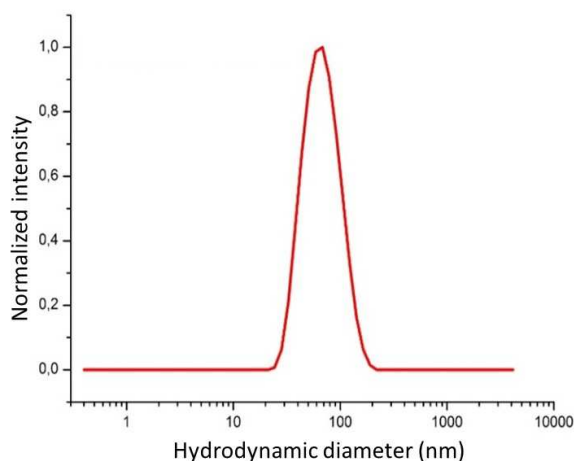
Fig. 1 - Distribution curve for the hydrodynamic diameter of \text{Fe}_3\text{O}_4 nanoparticles measured by the ultrasound spectrometer DT-100.
